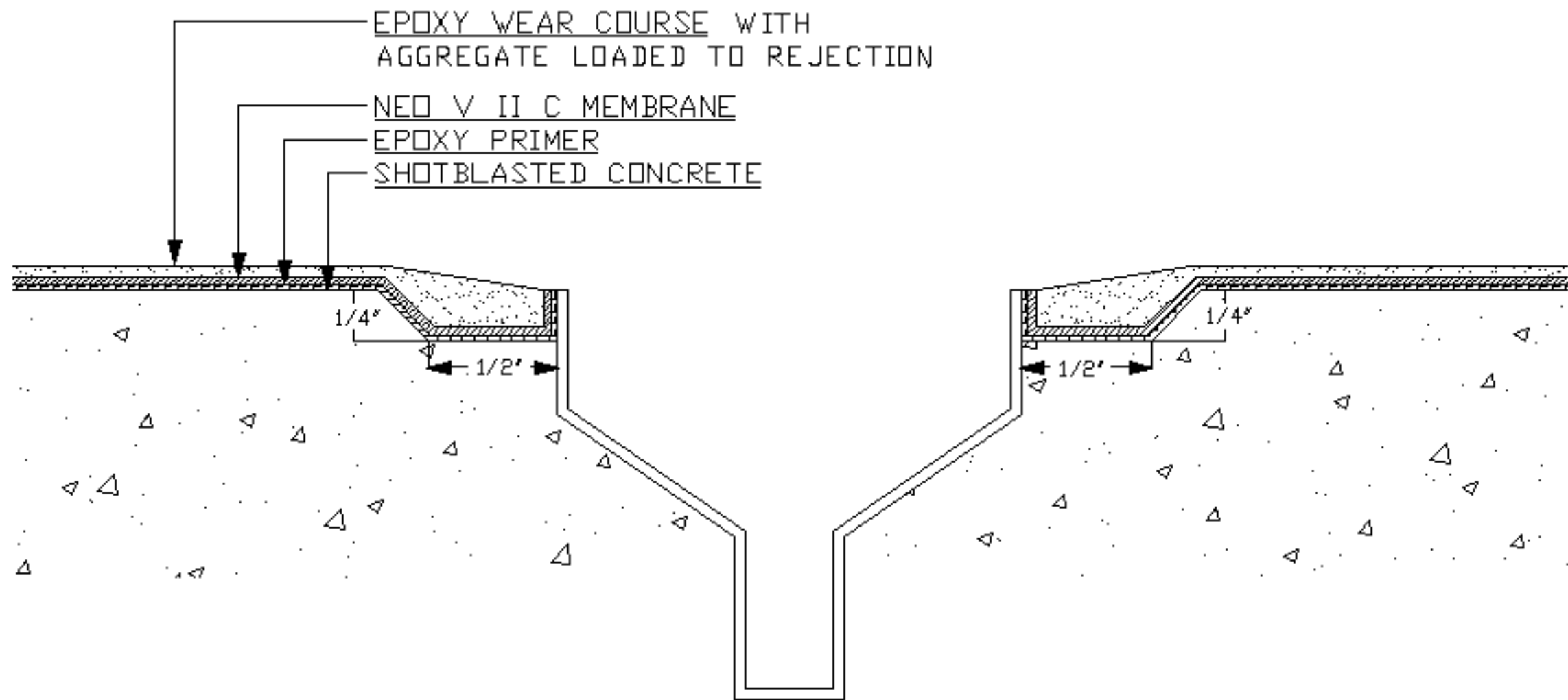
DETAIL AT FLOOR DRAINS
